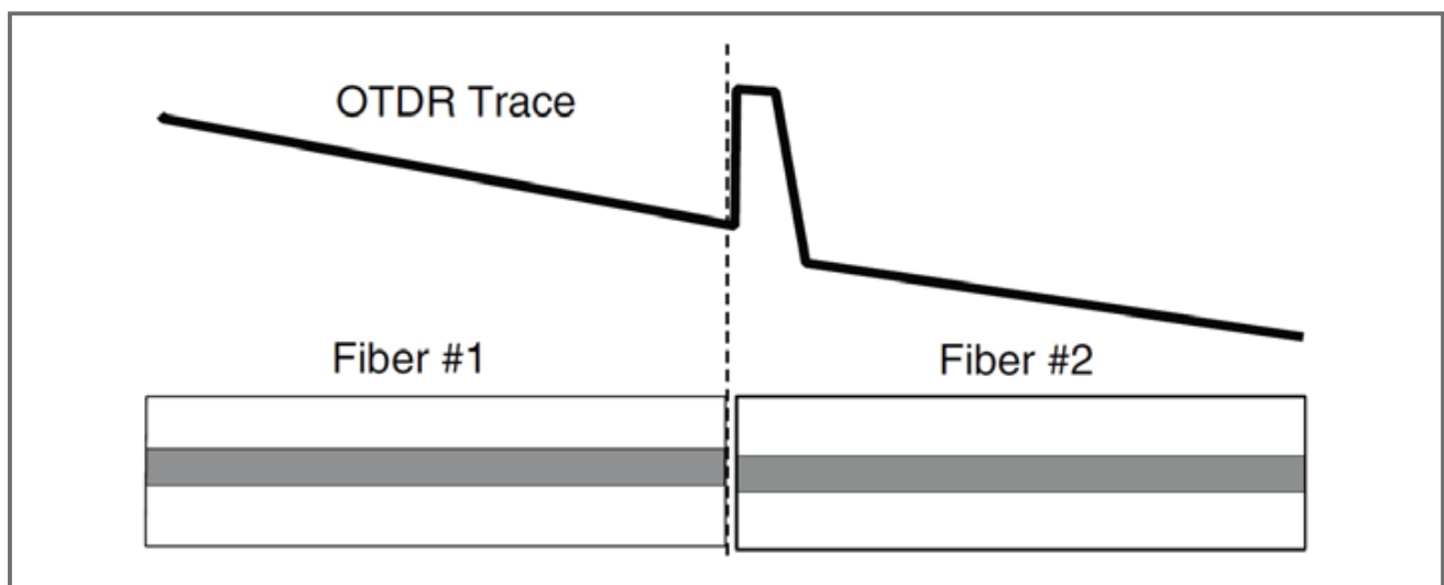
Figure 15 - Reflective Event Location
