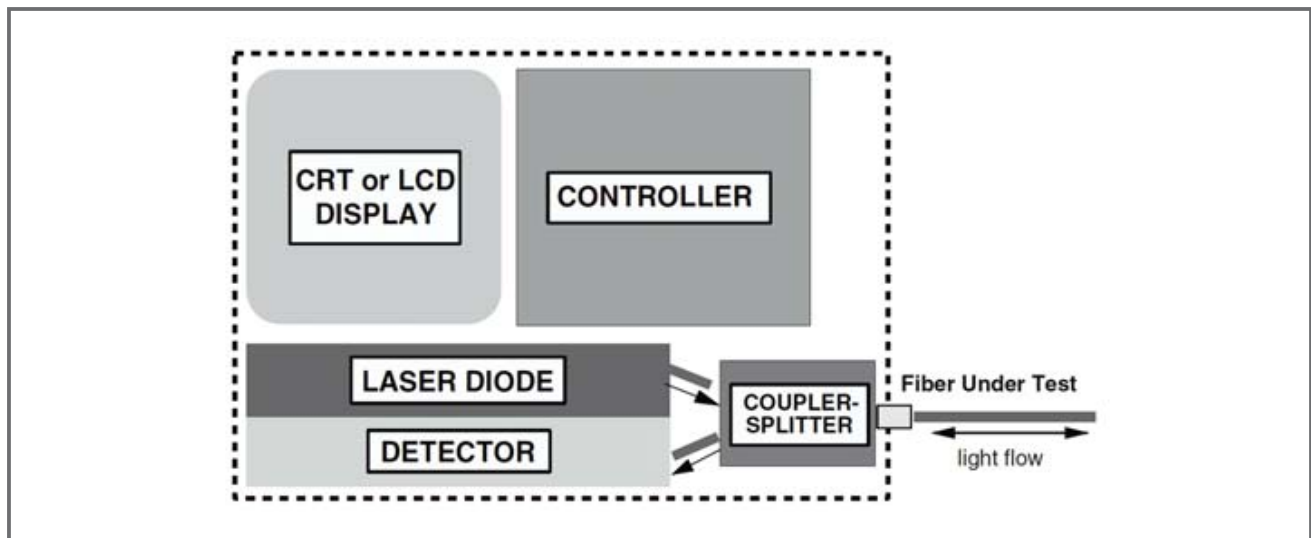
Figure 4 - OTDR Block Diagram
