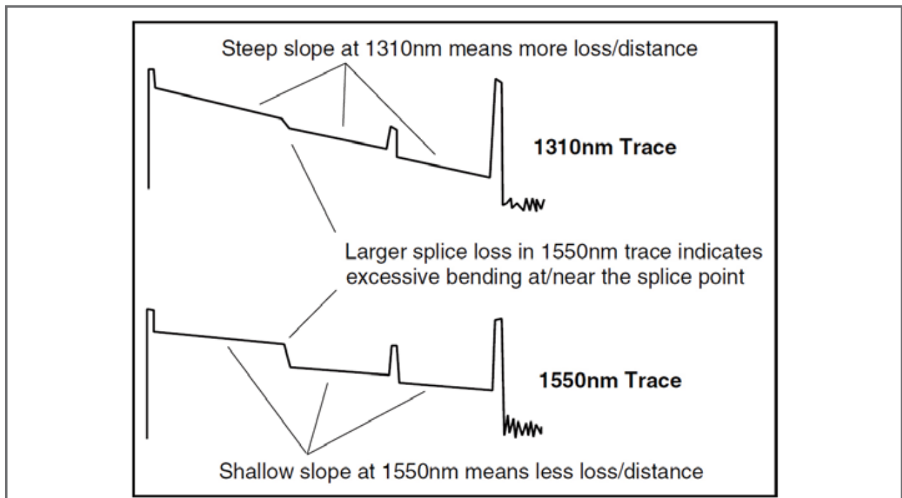
Figure 10 - Wavelength Differences
