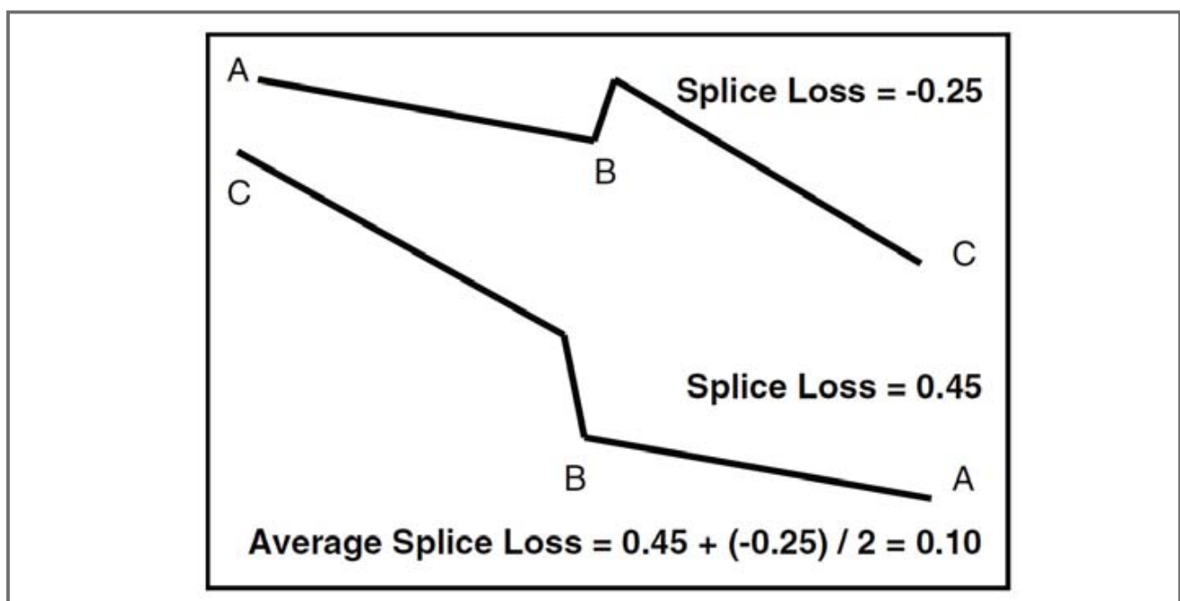
Figure 20 - Treatment of Gain Splices
