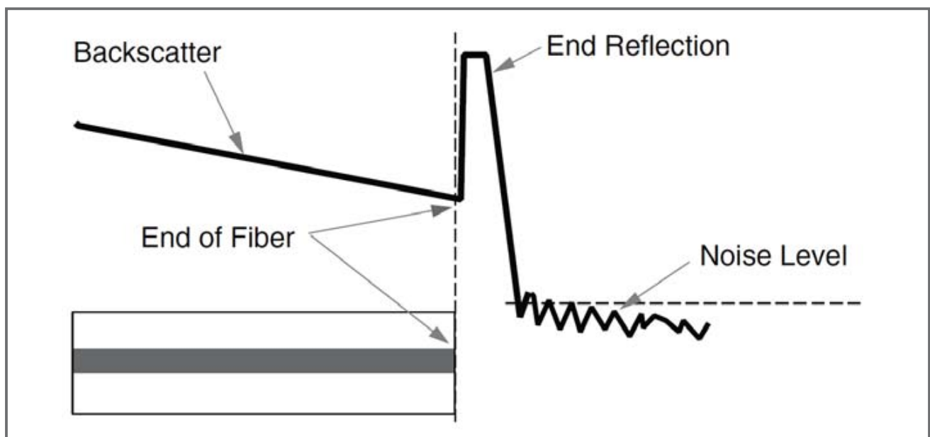
Figure 13 - Fiber End Location
