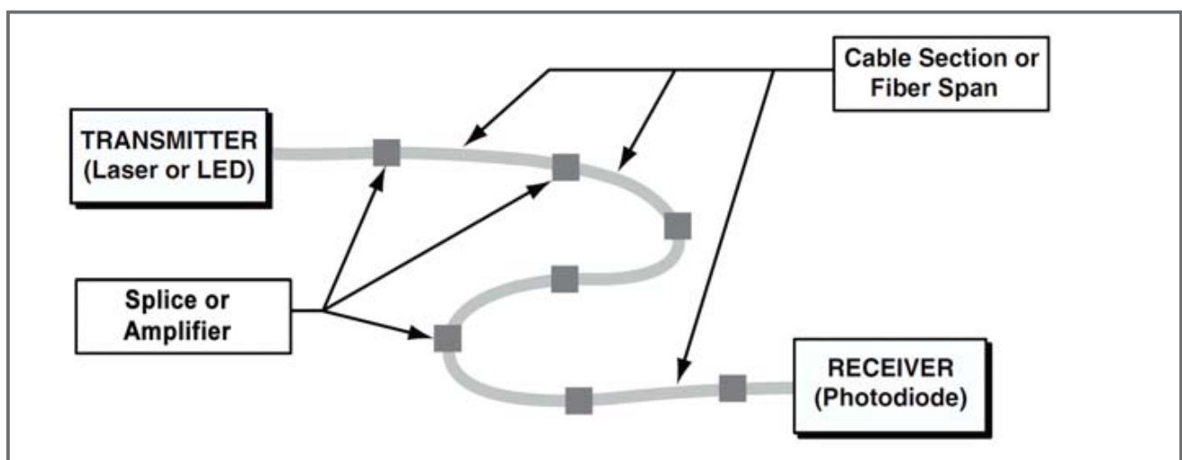
Figure 1 - Typical Fiber Optic Transmission System
