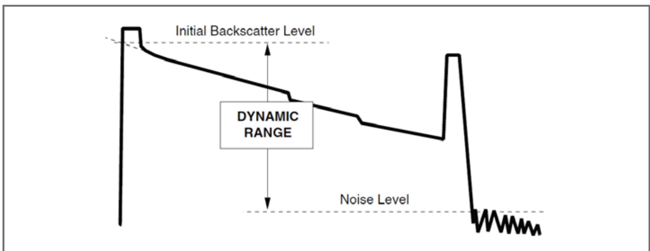
Figure 6 - Dynamic Range
