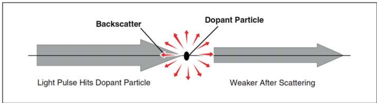
Figure 2 - Rayleigh Scattering
