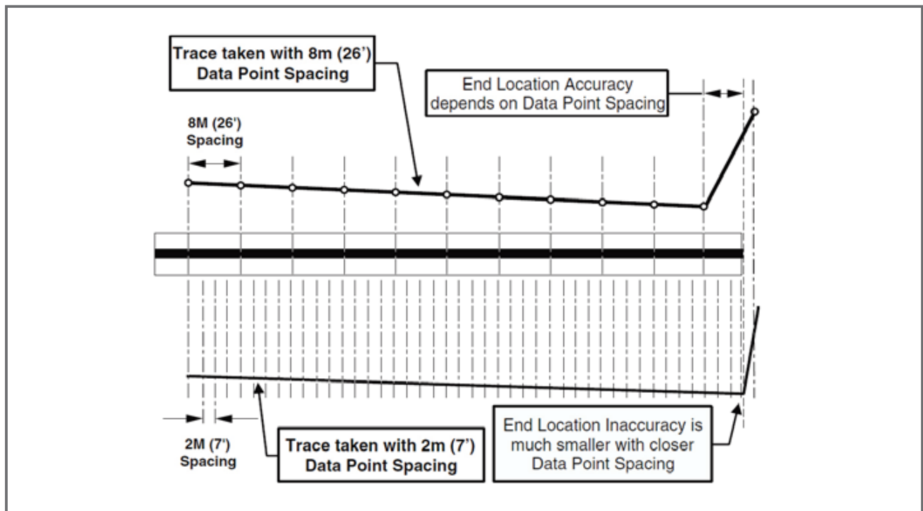
Figure 9 - Data Point Resolution
