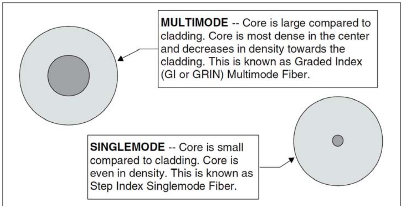
Figure 11 - Optical Fiber Types
