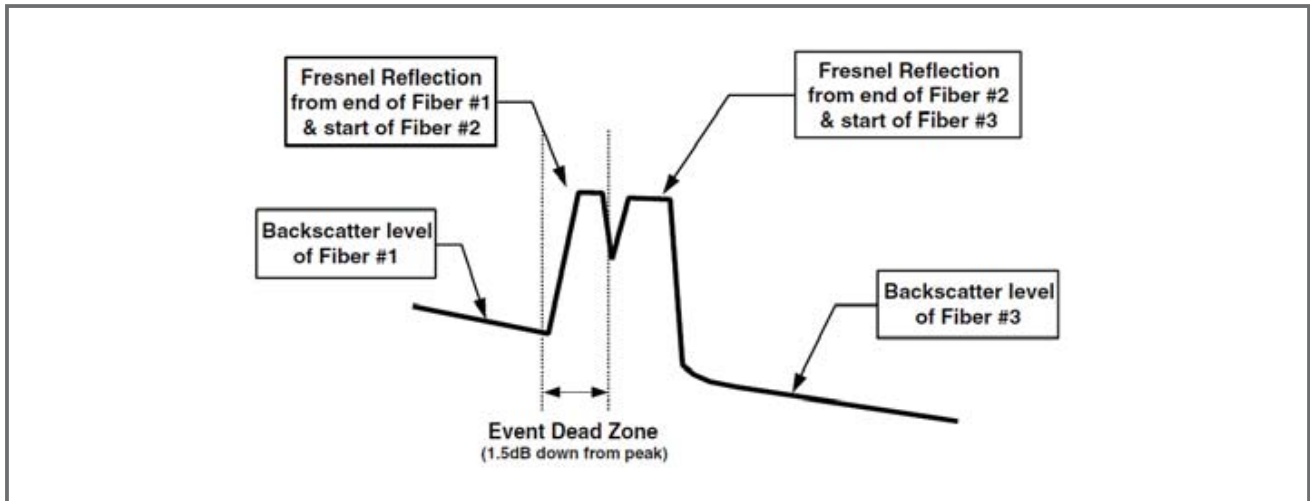
Figure 7 - Event Dead Zone
