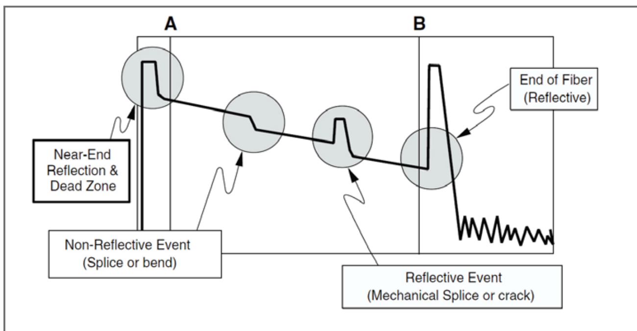
Figure 12 - Elements of an OTDR Trace
