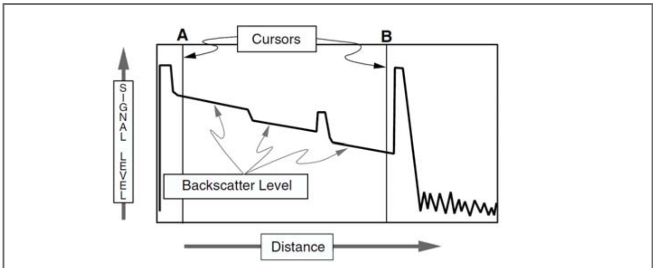
Figure 5 - Components of OTDR Trace Display
