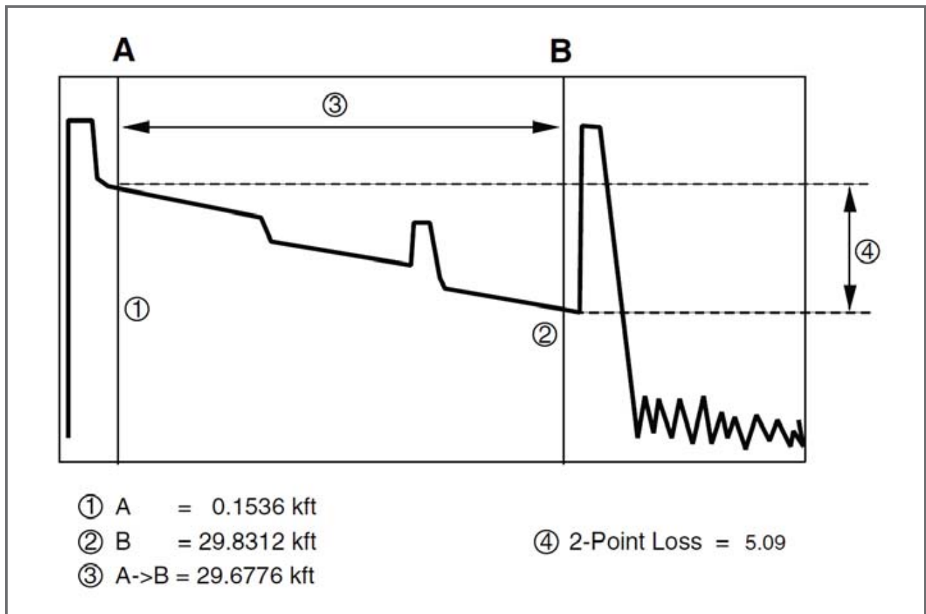
Figure 17 - OTDR Measurements Display
