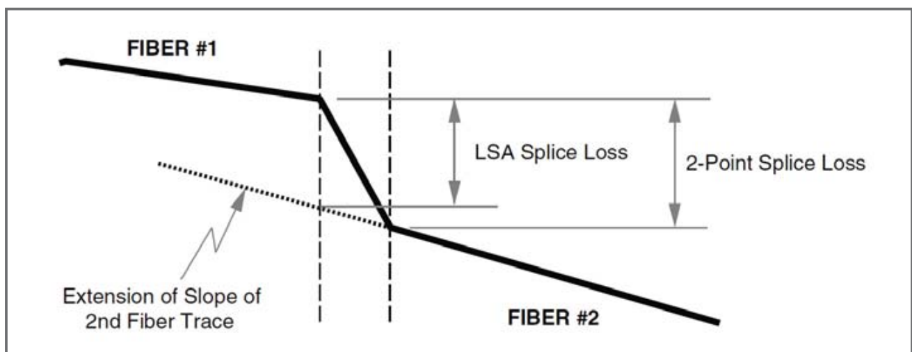
Figure 18 - LSA vs. 2-Point Splice Loss
