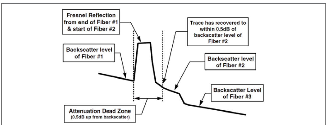
Figure 8 - Attenuation Dead Zone
