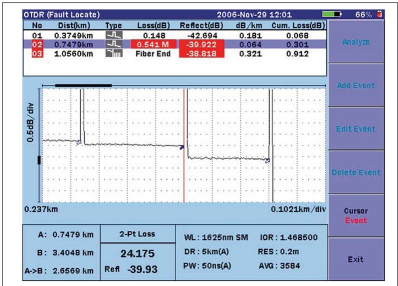
Figure 19 - Event Table Example
