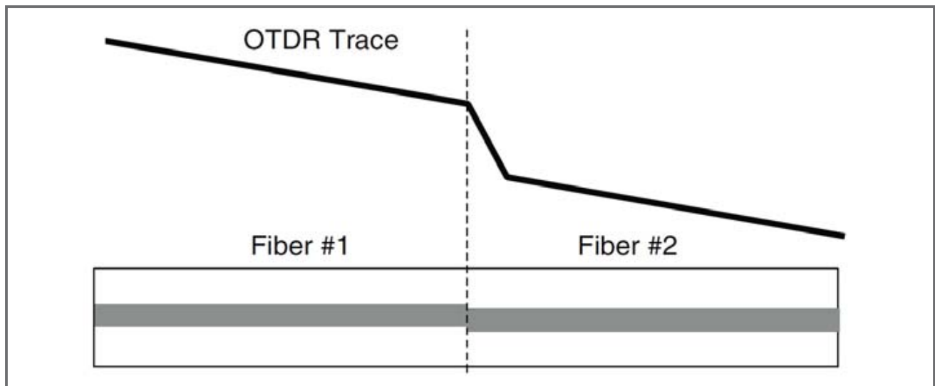
Figure 16 - Non-Reflective Event Location
